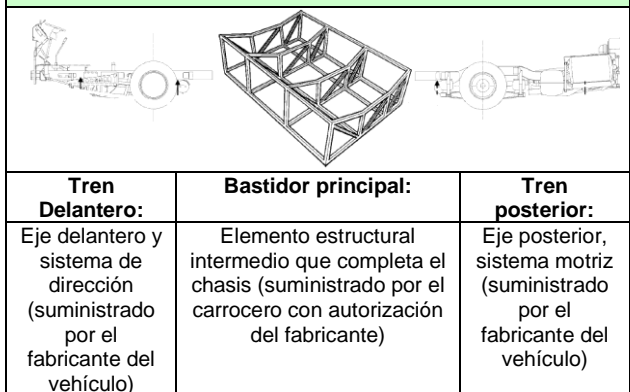
Figura II.2 : Ómnibus Integral
